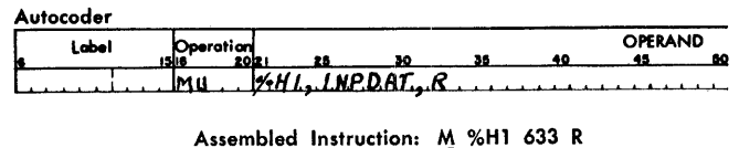
Figure I-24. Read Data
