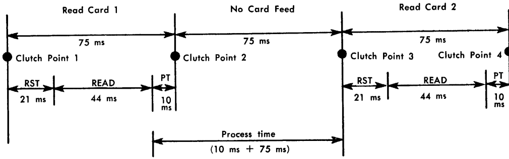
Figure I-96. 400 CPM Operation
